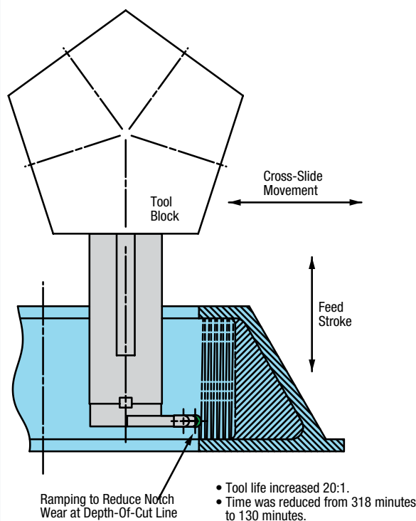
Figure 42 – Boring a Cavity with Ceramics
