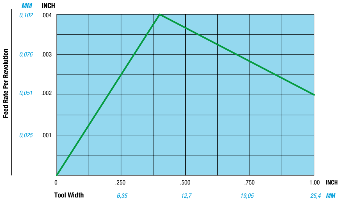
Figure 52 – Grooving Feeds vs. Tool Width
