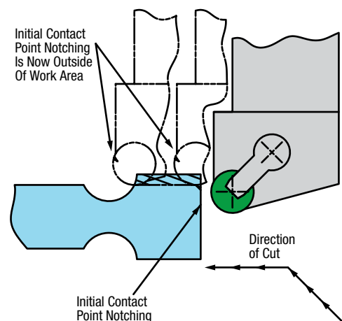
Figure 28 – Chamfering and Facing
