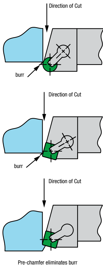
Figure 32 – Pre-Chamfer to Eliminate Burrs
