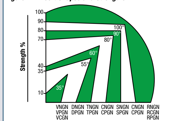
Figure 7 – Insert Shapes and Strengths
