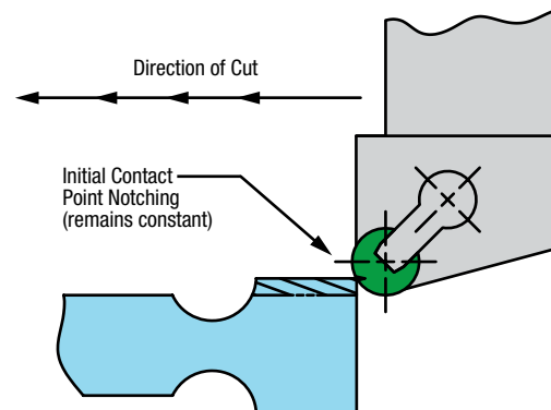
Figure 27 – Straight Facing
