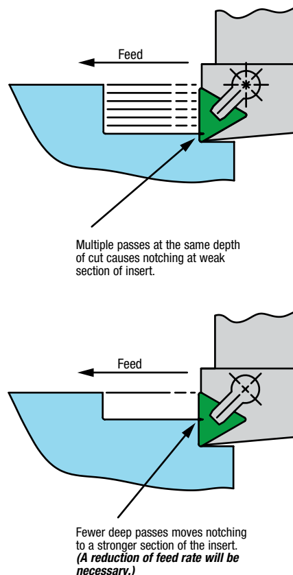
Figure 33 – Rethink Depth of Cut
