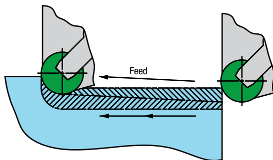
Figure 37 – Ramping/Negative Inserts/RNGN
