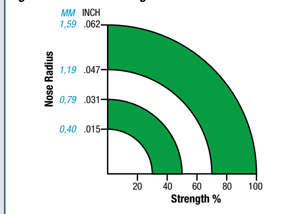
Figure 8 – Relative Strength for Various Insert Radii
