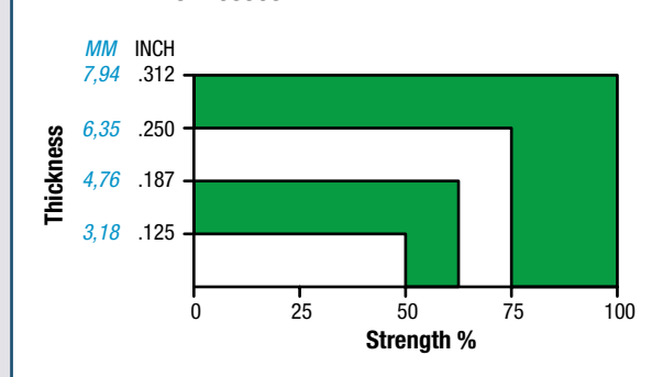
Figure 9 – Relative Strength for Various Insert Thicknesses
