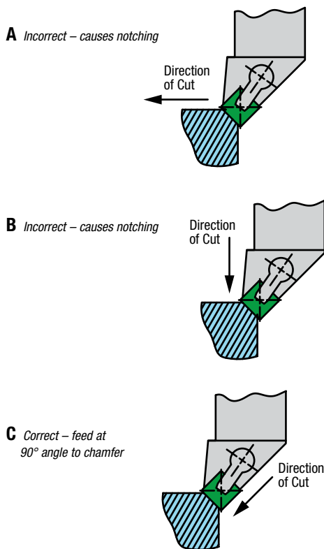
Figure 26 – Chamfering Techniques
