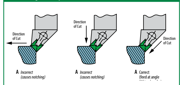
Figure 55c Chamfering Techniques
